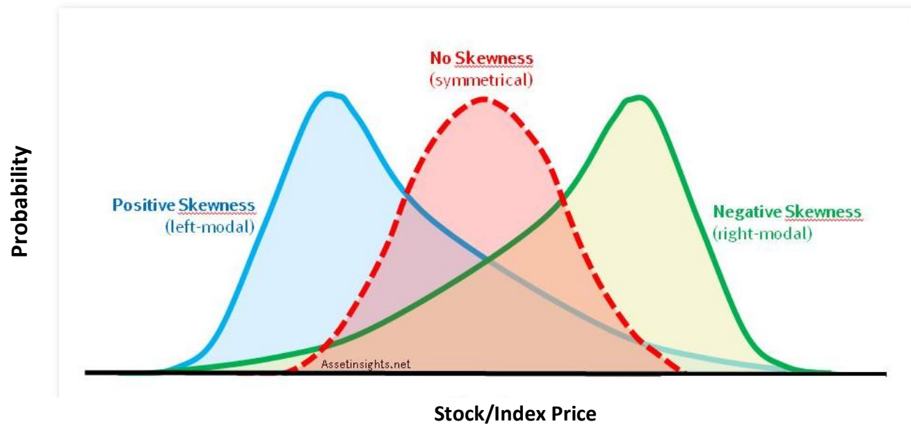
Probability Distributions with and without Skewness
